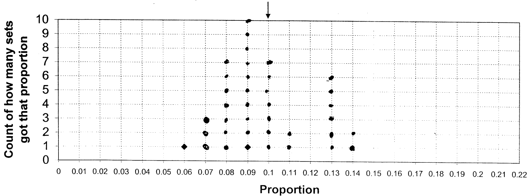
Proportion of 0's in 200 trials
